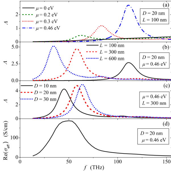
FIG. 4. Frequency dependence of the normalized absorption cross section \Lambda of the CNT at different (a) chemical potentials \mu \in \{0, 0.2, 0.3, 0.46\} eV, L = 100 nm, D = 20 nm, (b) tube lengths L \in \{100, 300, 600\} nm, \mu = 0.46 eV, D = 20 nm, and (c) outer diameters D \in \{10, 20, 30\} nm, \mu = 0.46 eV, L = 300 nm. (d) The conductivity spectrum of the film comprising identically B-doped CNTs with diameter of 20 nm and length distribution as in Fig. 1(b); CNT volume fraction is 20%, N = 14 and \mu = 0.46 eV.
